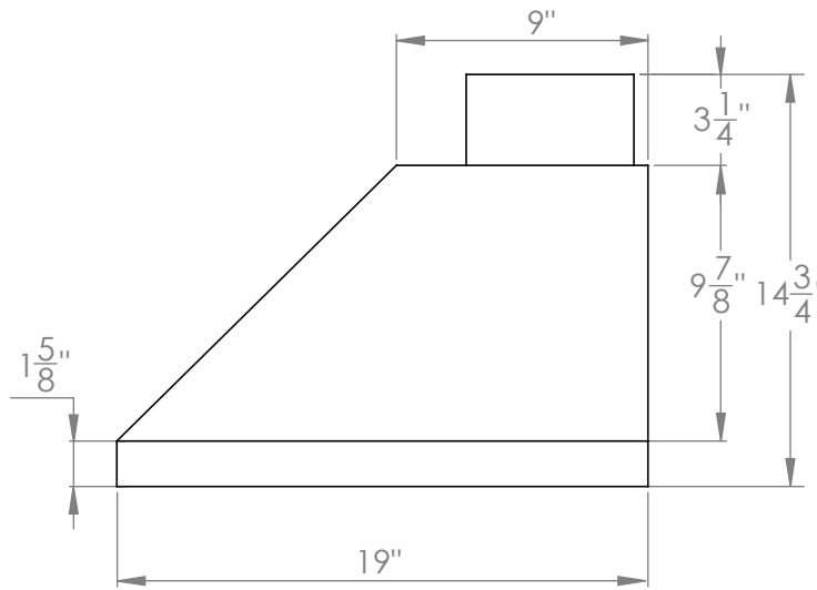
SIDE
